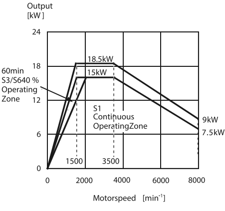
ME-1690/1890/1611/1811/2012 Fanuc-Drive
