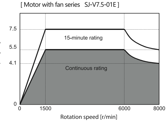
ME-1370/1470/1670/1690/1890/1611/1811/2012 Mitsubishi-Drive
