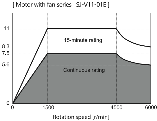
ME-1060/1160/ 1260/1270 Mitsubishi-Drive
