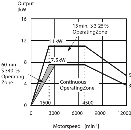
ME-655/855/1055 Fanuc-Drive
